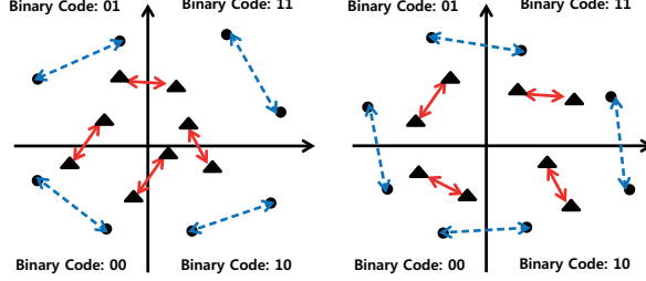
Fig. 2. Pairs of triangles connected by red solid lines are similar ones and pairs connected by blue dotted lines are dissimilar ones in the original space. Both embeddings well preserve locality, however, similarities in the Hamming space are not preserved after binary quantization (left panel), while similarities are still preserved even after binary quantization (right panel). A proper rotation by minimizing the quantization error improves the performance, as demonstrated in [9].
